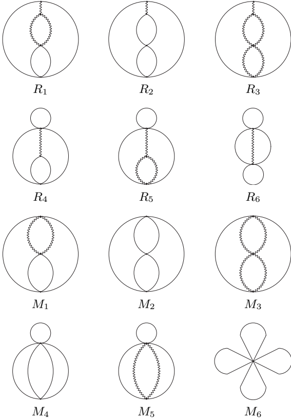
Fig. 1. List of independent topologies belonging to the n_f^2 contribution. The topologies R_1 – R_6 are reducible, whereas the topologies M_1 – M_6 are master integrals. The wavy and solid lines depict massless and massive propagators respectively
